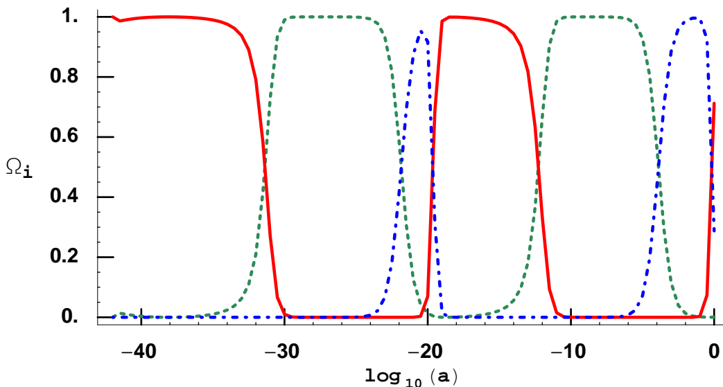
Figure 3: The cosmological history of Model 2. Shown are the relative energy density fractions in radiation (green/dashed), matter (blue/dot-dashed), and the noncanonical scalar (red/solid), as a function of the logarithm of the scale factor.
