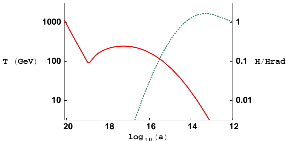
Figure 4: The temperature history of Model 2 (red/solid) near the electroweak phase transition. Shown in green/dashed is the Hubble parameter H of Model 2 normalized to the expansion rate H_{\text{rad}} for pure radiation.
